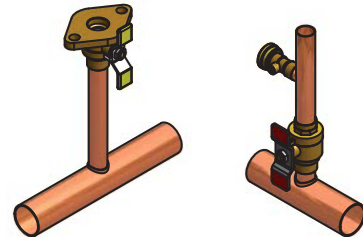
NHB Series Secondary Supply & Return Manifolds (#GFFM-SKTZUS-001)
