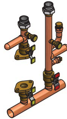
NHB Series Primary Manifold (#GFFM-MSOZUS-001)
