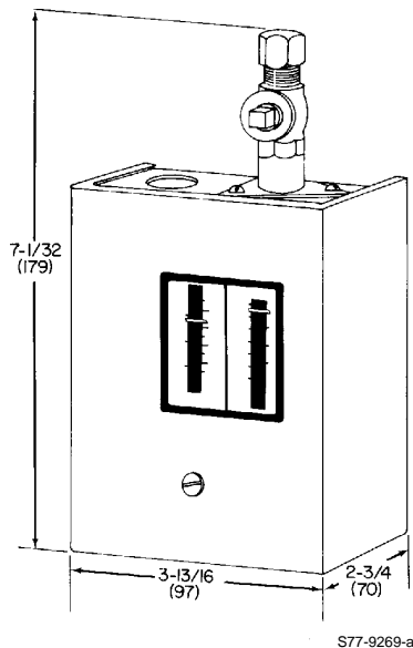
P643A Dimensions in Inches (Millimeters)
