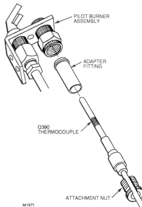
Fig. 3—Installing thermocouple with attachment nut.
