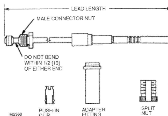
Fig. 1—Q390 installation.
