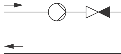
Fig. 4 Non-return valve
