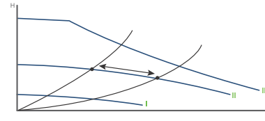
Fig. 19 Three constant-curve/constant-speed settings
